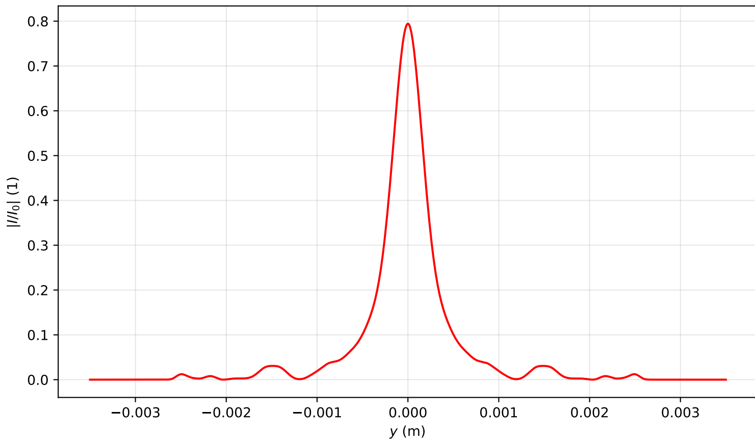
Intensity profile I(x=0, y, z=2.866)/I_0 , P_{in}=4.0P_{cr} , artificial time
